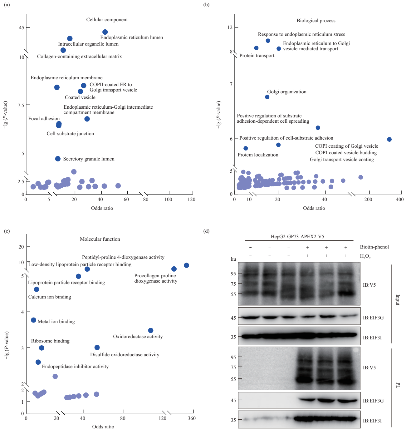
Fig. 3 Results of GO enrichment analysis of GP73 interacting proteins
