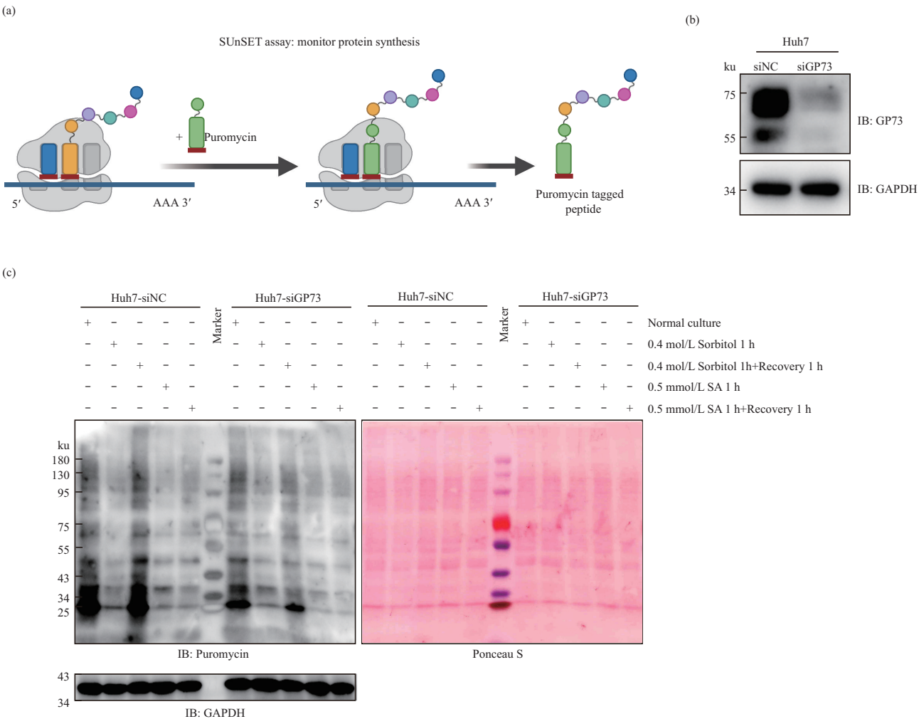
Fig. 4 GP73 promotes translational rates in hepatocellular carcinoma cells
