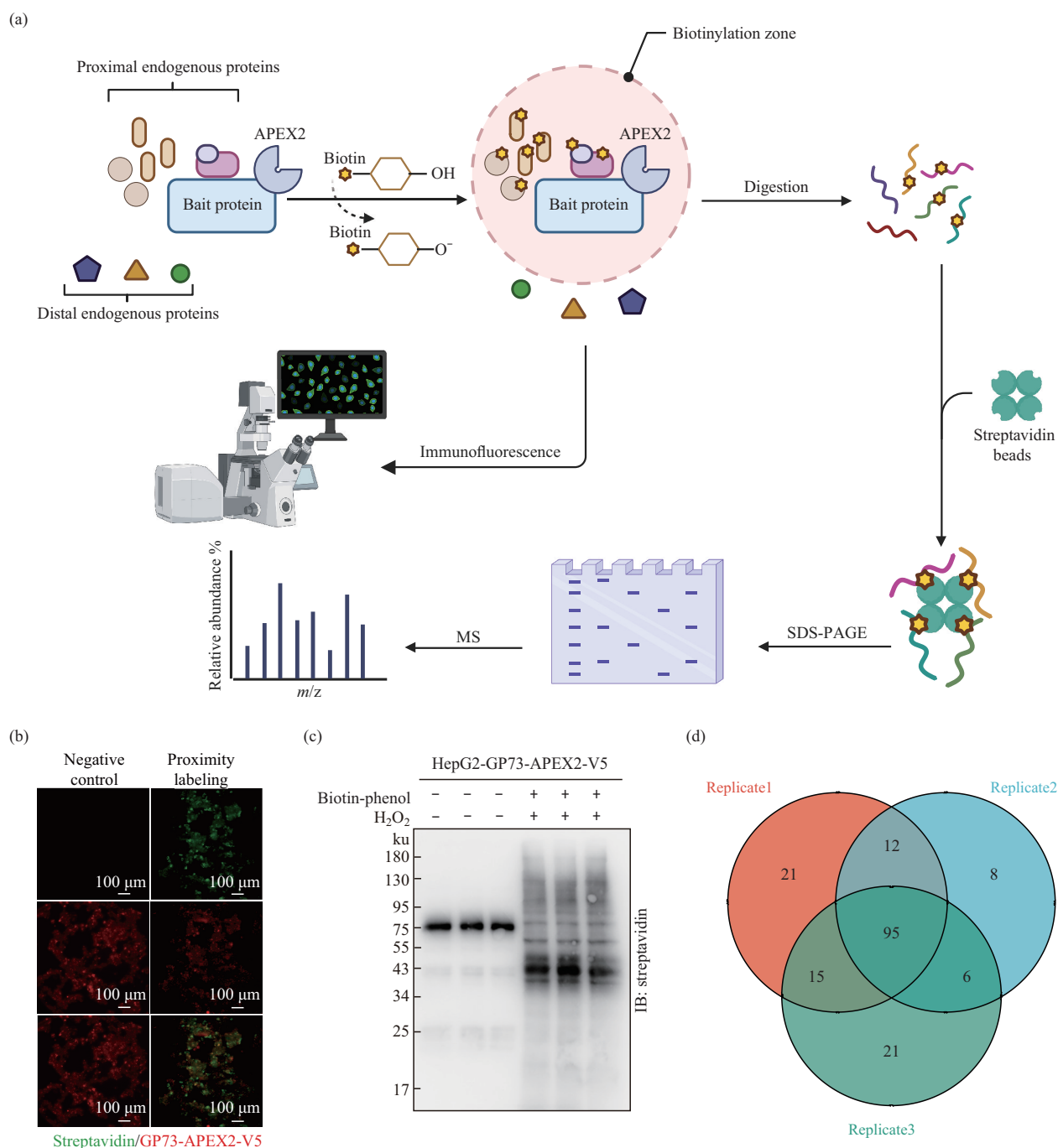
Fig. 2 Results of proximity labeling experiments
