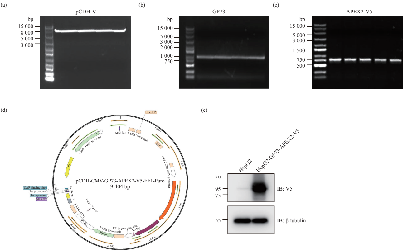
Fig. 1 Establishment of HepG2-GP73-APEX2-V5 stable cell line
