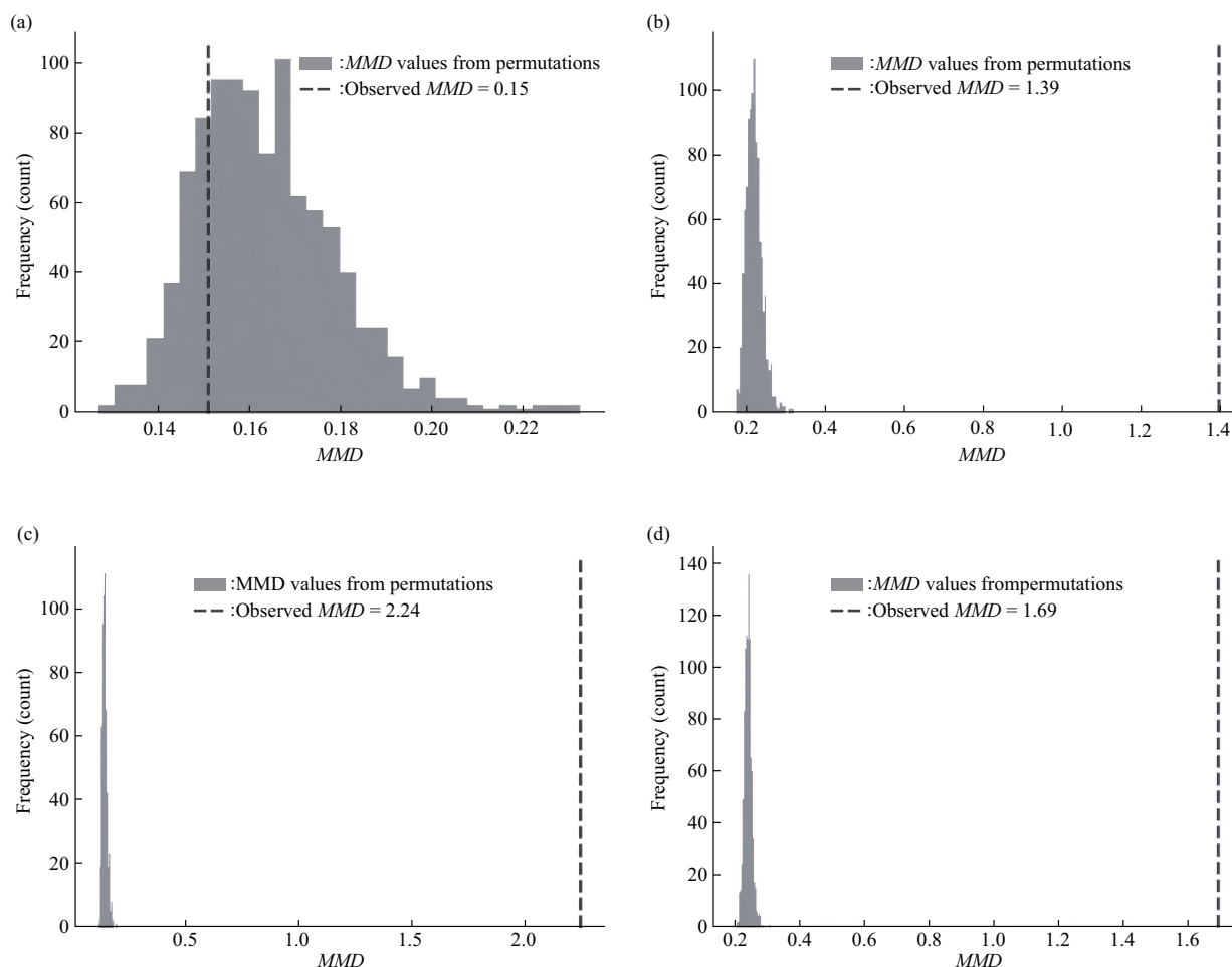
Fig. 2 Analysis of differences in dataset distribution
