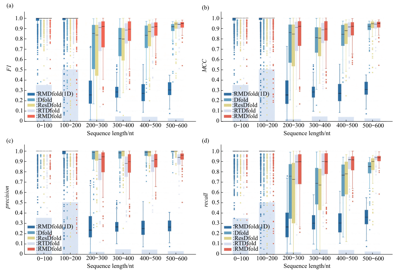
Fig. 3 Visualization of prediction metrics for different average sequence lengths ranges in the ablation experiments
