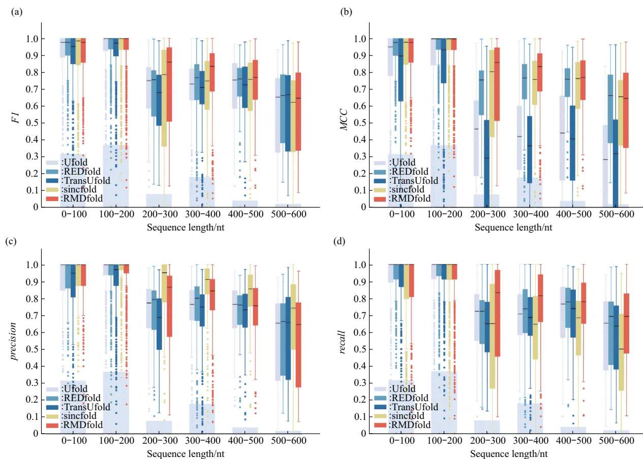
Fig. 6 Visualization of prediction metrics for different average sequence lengths ranges on the ArchiveII dataset
