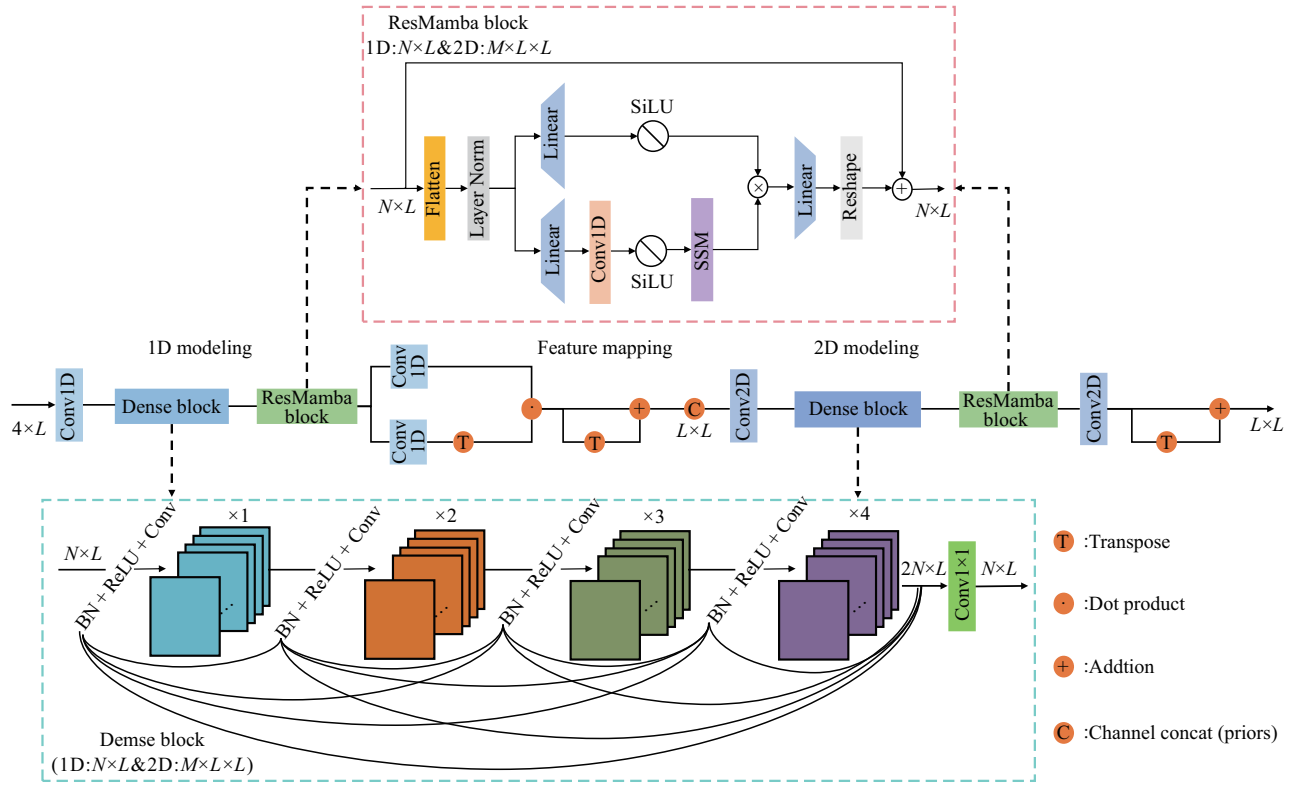
Fig. 1 The proposed RMDfold model
