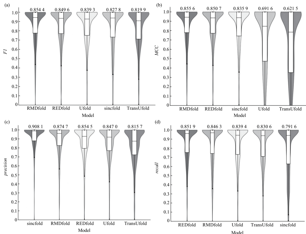
Fig. 5 Visualization of prediction metrics of different methods on the ArchiveII dataset (a) F1 , (b) MCC , (c) precision , (d) recall .
