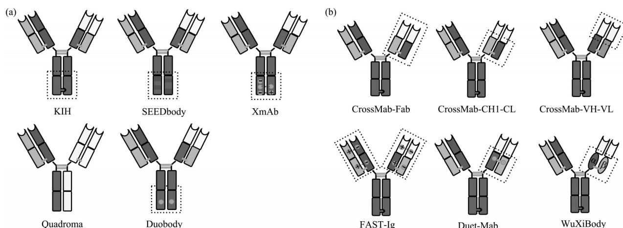
Fig. 2 The design of asymmetric bispecific antibody
