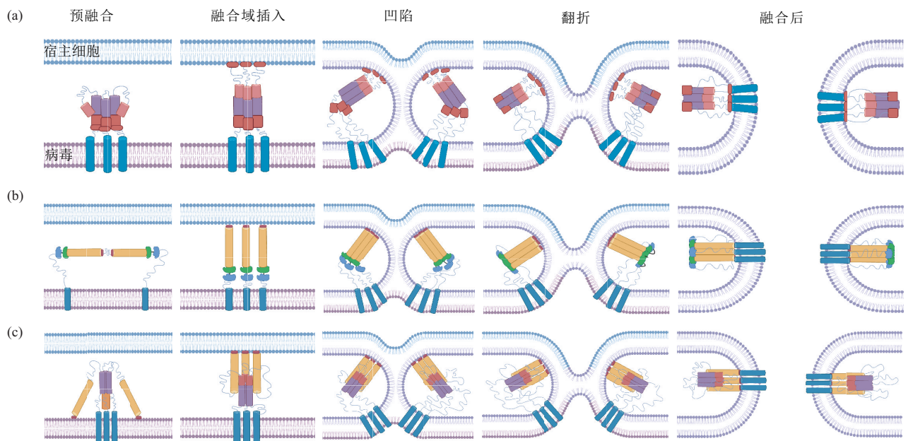
Fig. 1 Structural modeling of key domains in three classes of viral membrane fusion proteins across distinct conformational states during fusion
