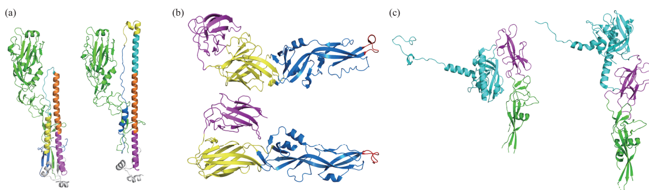
Fig. 2 Representative pre-fusion and post-fusion structural conformations of three classes of viral membrane fusion proteins
