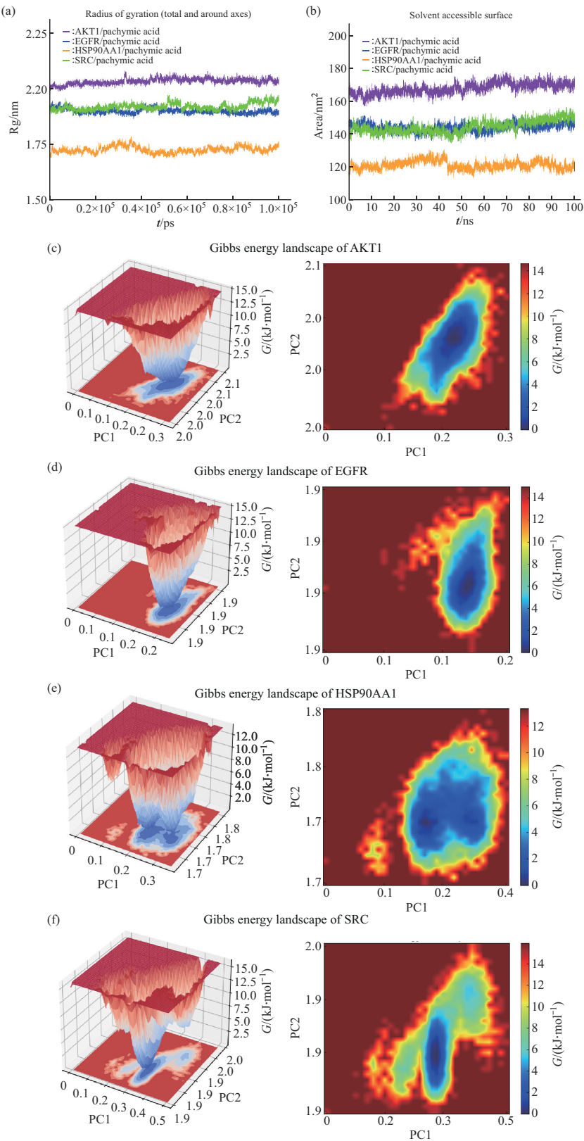
Fig. 4 Molecular dynamics simulation results of PA-target complex
