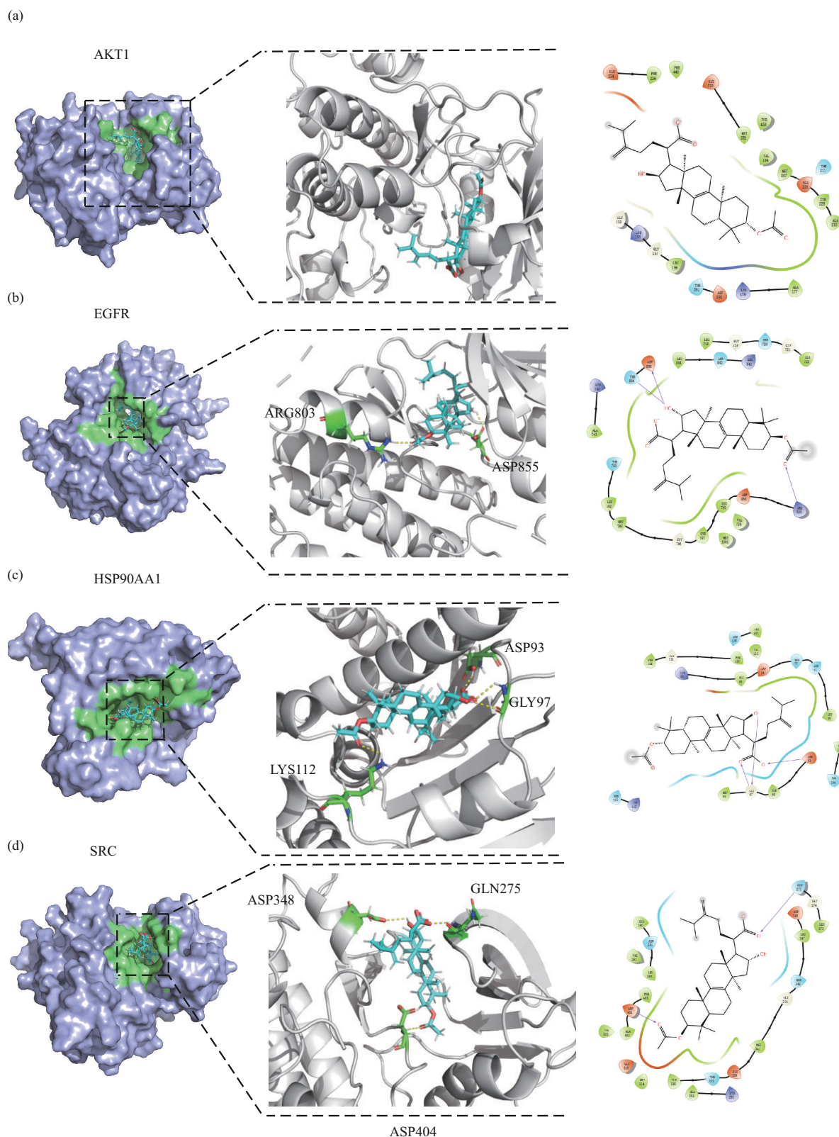
Fig. 2 Pictorial representation of the molecular interactions between cerevisterol and the top 4 targets
