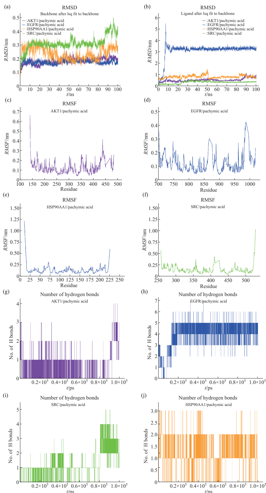
Fig. 3 Molecular dynamics simulation results of PA-target complex
