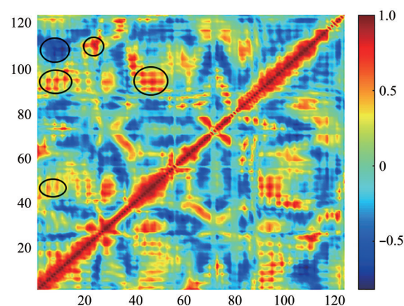
Fig. 3 Average residue cross-correlations for human 31 sPLA 2 -IIA members
