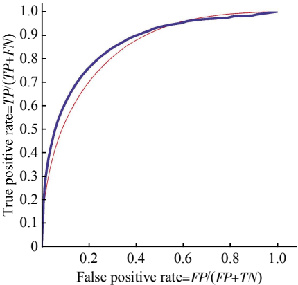
Fig. 2 ROC curves of NetTurnP and BTMapping on EVA937 dataset —: NetTurnP; —: BTMapping.
