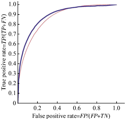
Fig. 1 ROC curves of NetTurnP and BTMapping on BT426 dataset —: NetTurnP; —: BTMapping.
